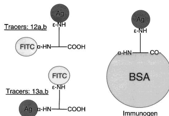
Figure 2. Schematic representation of the structural homology appearing between immunogen and tracers 12a,b and the structural heterology between immunogen and tracers 13a,b . Immunogen and tracers 12a,b have the antigen (2,4D or 2,4,5T) attached to the amino group of the \epsilon -primary aliphatic carbon atom of L-lysine. Tracers 13a,b have the antigen attached to the aminogroup of the \alpha -secondary asymmetric carbon atom of L-lysine.
