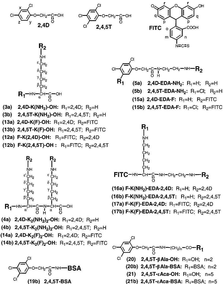
Figure 1. Chemical structures of synthesized derivatives, tracers, and immunogens. For each compound a code number (in parentheses) and a short name (with boldface letters) are given. The short name has been chosen to describe the corresponding chemical structure. When an R group is noted as 2,4D or 2,4,5T, it represents their acyl derivatives. When R is given as FITC, it represents the thiocarbamoyl fluorescein. The notation with Greek characters in L-lysine and with Latin characters in 2,4D and FITC is used for the study of the 1 H NMR chemical shifts and for the study of the Figures S1–S4 of the Supporting Information. Replacing the two chlorine atoms from 15a with two bromine atoms can confirm the structure of tracer 15c .
