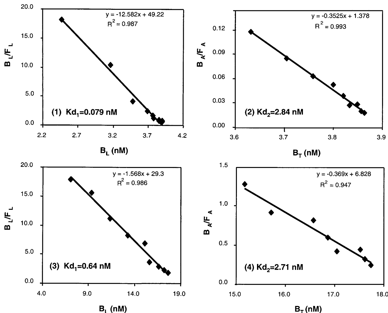
Figure 4. Scatchard plots from experiments "A" (graphs 1 and 2) and "C" (graphs 3 and 4). The equations given in graphs 1 and 3 correspond to the scatchard equation B_L/F_L = -(1/K_{d1})B_L + R_0/K_{d1} for determination of the K_{d1} values, when 2,4D is not present in the reaction mixture ( y = B_L/F_L , x = B_L , and R_0 = total antibody concentration). The equations given in graphs 2 and 4 correspond to the scatchard equation B_A/F_A = -(1/K_{d2})B_T + R_0/K_{d2} for determination of the K_{d2} value ( y = B_A/F_A , x = B_T , and R_0 = total antibody concentration).
