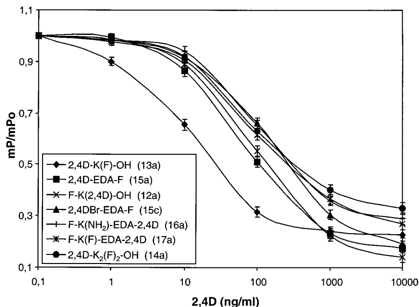
Figure 3. Standard curves obtained using the monoclonal antibody E2/G2 and the 2,4D tracers 13a , 15a , 12a , 15c , 16a , 17a , and 14a . In all cases, mP_0 was approximately 150. Each standard curve was the mean of four curves obtained from separate experiments. The error bars presented in the graphs are \pm 1 SD.
